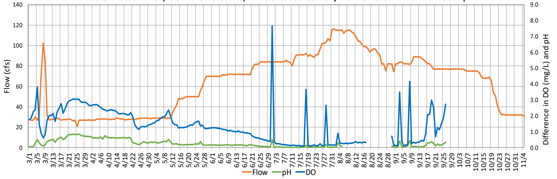
East Fork Russian River (Below Lake Mendocino) - Difference between Daily Maximum and Minimum for DO and pH
