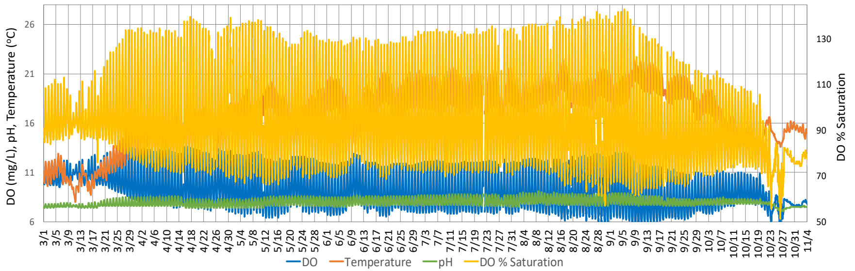
Hopland Water Quality Trend
