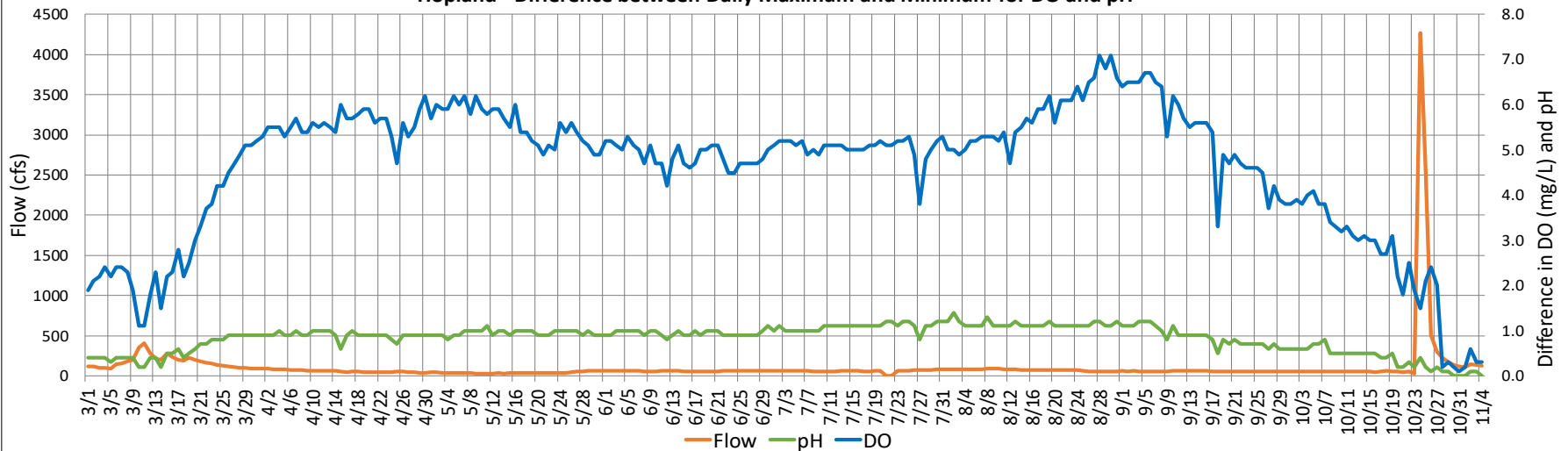
Hopland - Difference between Daily Maximum and Minimum for DO and pH
